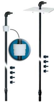
48" Drum & Tote Stick Comes with a Hastelloy strainer, check valve, and a variety of hose barbs - Viton or EPDM.
